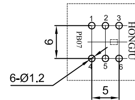
PCB HOLE( BOTTON VIEW)
